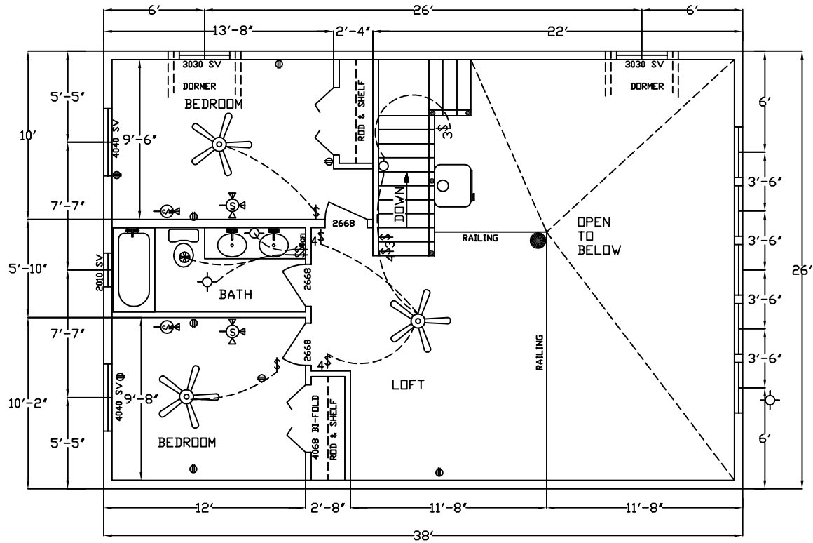
LOFT FLOOR PLAN 572 SQ. FT.
