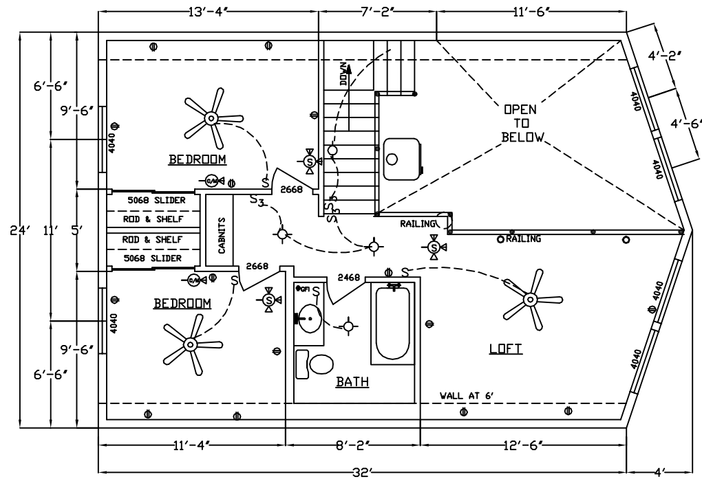
LOFT FLOOR PLAN 654 SQ. FT.
