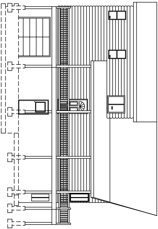
LEFT ELEVATION
