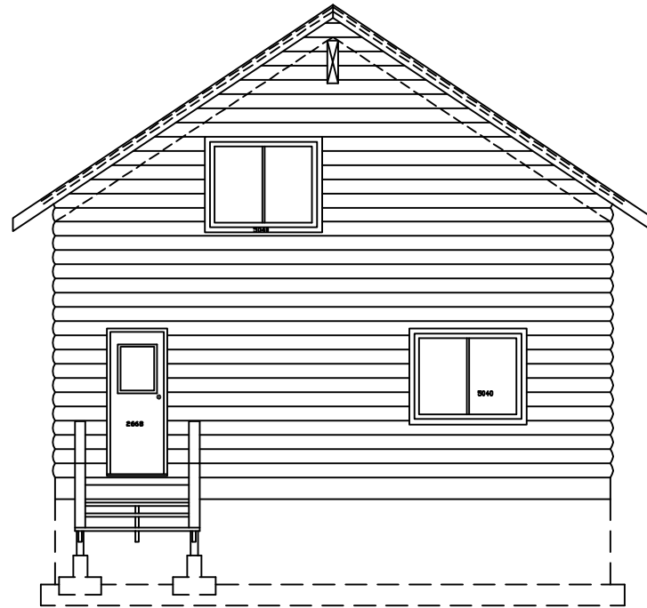
REAR ELEVATION
