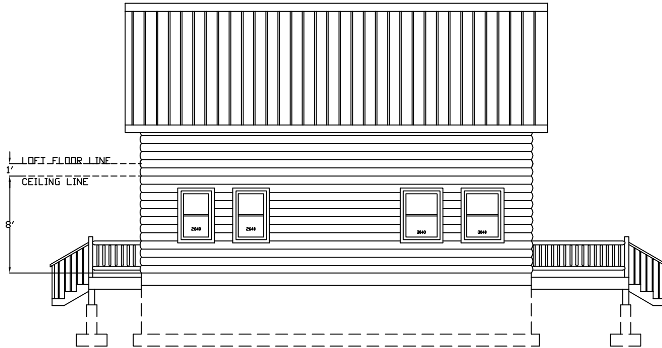
LEFT ELEVATION
